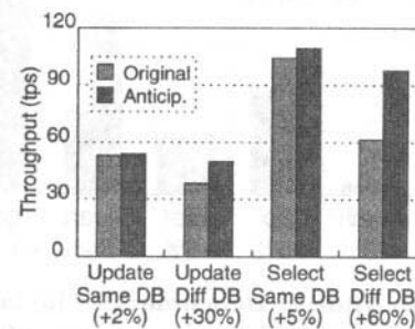
Figure 11: The TPC-B database benchmark and variants: two clients issuing update versus select queries into the same versus different databases.
