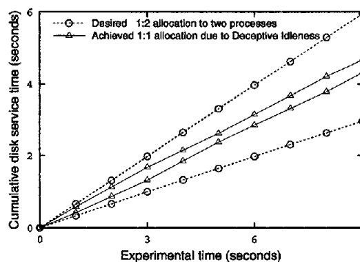
Figure 1: A proportional-share scheduler: The outer pair of lines denote ideal scheduler response to an allocation ratio of 1:2 to the two processes. Inner pair of lines: synchronous I/O causes requests to be almost alternately serviced from the two processes, yielding proportions much closer to 1:1.
