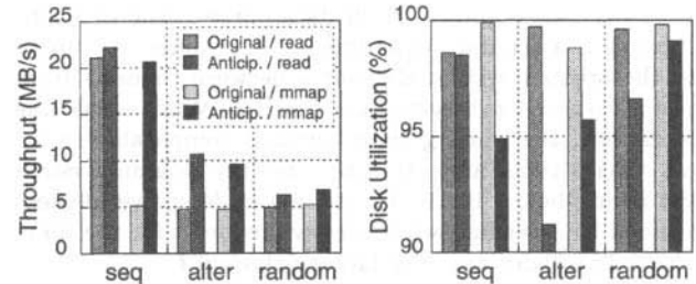
Figure 4: Impact of anticipatory scheduling on disk throughput and utilization, using sequential, alternate-block and random access workloads, and read versus mmap based access.
