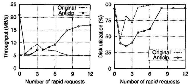
Figure 7: Adversary application
