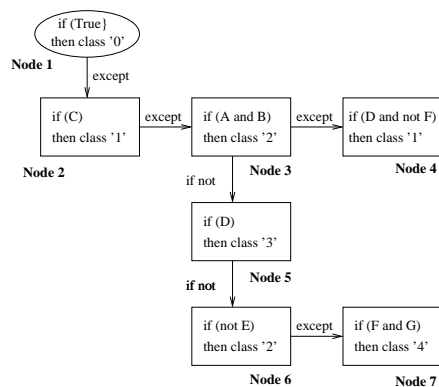
Fig. 1. An example SCRDR tree. Node 1 is the default node. A case for which only 'A' is true, it is classified as '0' by node 1. If only A, B, and C are true, it is classified as '2' by node 3, while it is classified as '1' by node 4 if on top of A,B, and C also D was true. If only 'A, C, and D are true it is classified as '3' by node 5. If only A and C are true, the case is classified as '2' by node 6, etc
