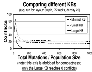
Figure 4: The “minimal” KB and “small” KB are unable to solve problem. The more mature KB can solve it effectively.
