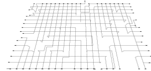
Figure 6: Solution to Burstein’s switchbox problem.
