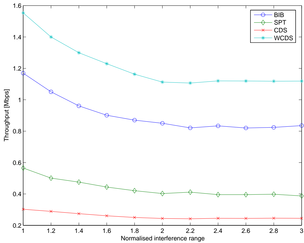
Figure 21: Impact of interference range on the throughput for BIB, WCDS, SPT and CDS. Number of nodes = 100.
