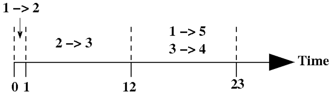
Figure 3: Alt_2 : Transmission schedule if each node can broadcast a packet more than once.
