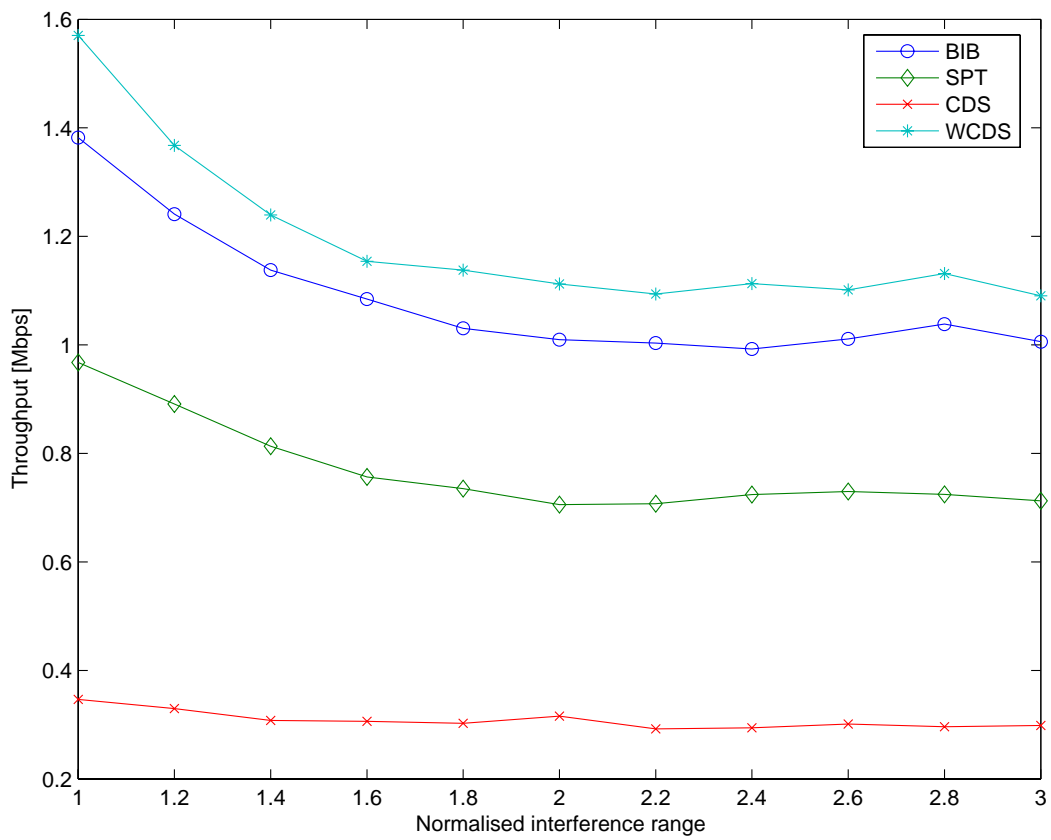
Figure 19: Impact of interference range on the throughput for BIB, WCDS, SPT and CDS. Number of nodes = 30.
