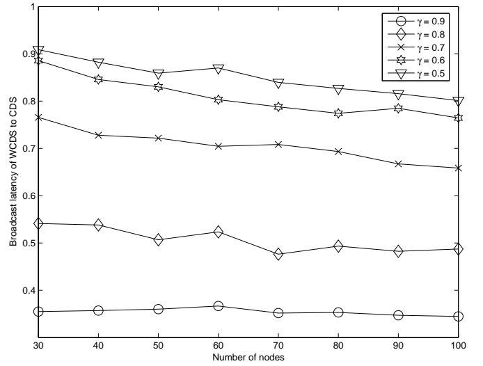
Fig. 6. This graph shows the geometric mean of the latency of WCDS to CDS over 100 randomly generated topologies of each network size.
