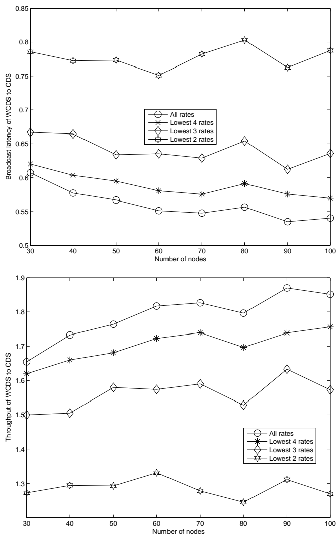
Fig. 8. Performance of WCDS algorithm (relative to CDS) using different number of transmission rates. The top graph shows latency while the bottom one shows throughput.
