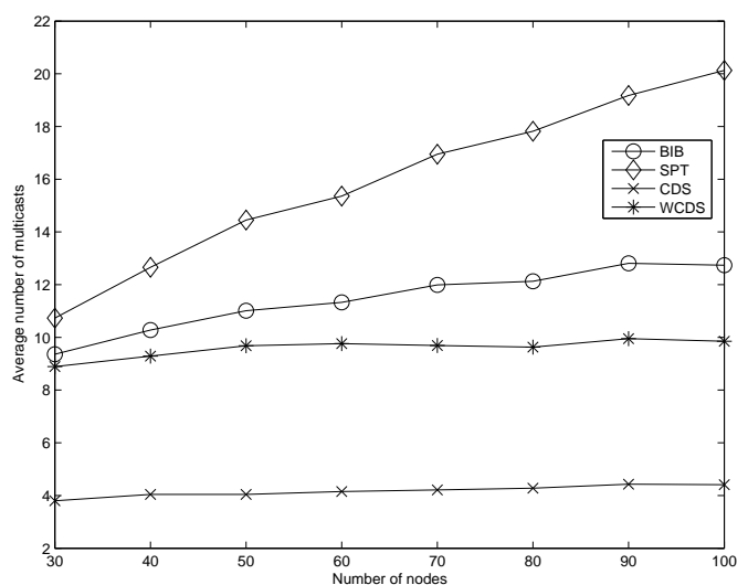
Fig. 5. This graph shows the mean number of multicasts per tree for BIB, WCDS, SPT and CDS.
