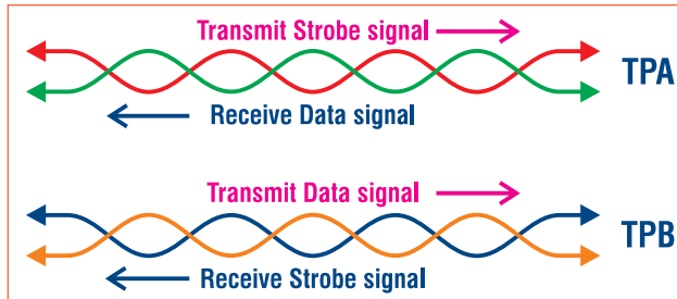
Fig.3: The Strobe and Data signals are sent along the IEEE 1394 bus via two shielded twisted-wire pairs, TPA and TPB.
