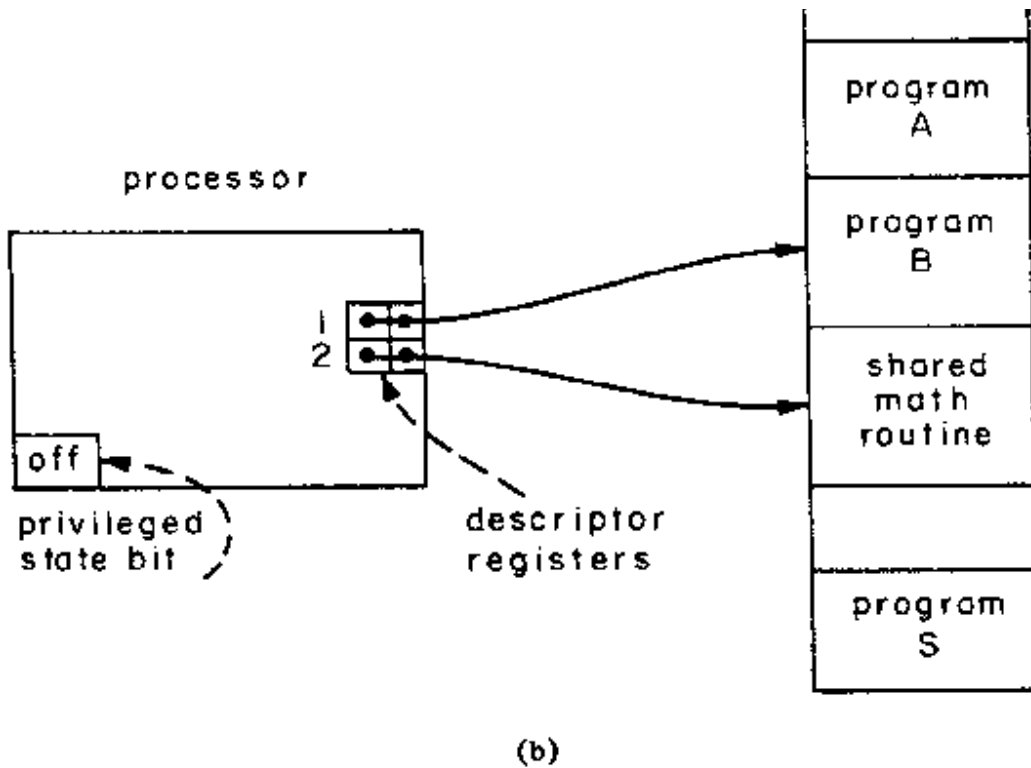
Fig. 2. Sharing of a math routine by use of two descriptor registers. (a) Program A in control of processor. (b) Program B in control of processor.
