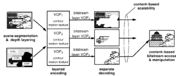
Object Based MPEG-4 Video Verification Model
