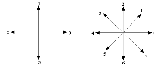
Direction numbers for 4-directional chain code Direction numbers for 8-directional chain code
