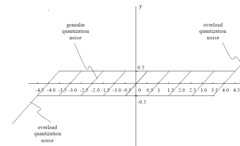
Quantization noise of the uniform mid-tread quantizer
