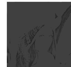
Entropy = 1.44. bits/pixel
