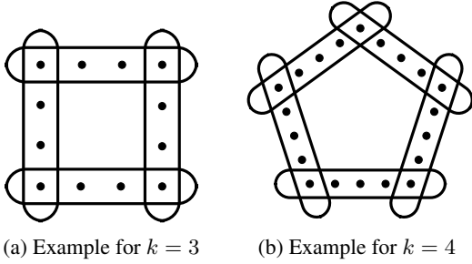
Figure 1: A visualization of the profiles used in Example 1. Dots represent voters and boxes represent candidates; candidates are approved by voters contained in the respective boxes.
