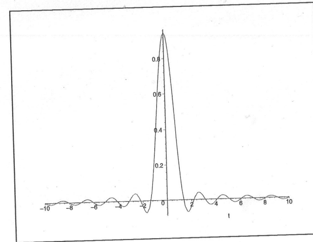
FIGURE 2. The PSWFs \varphi_0 with parameter values \sigma = \pi and \tau = 1 on a larger interval.
