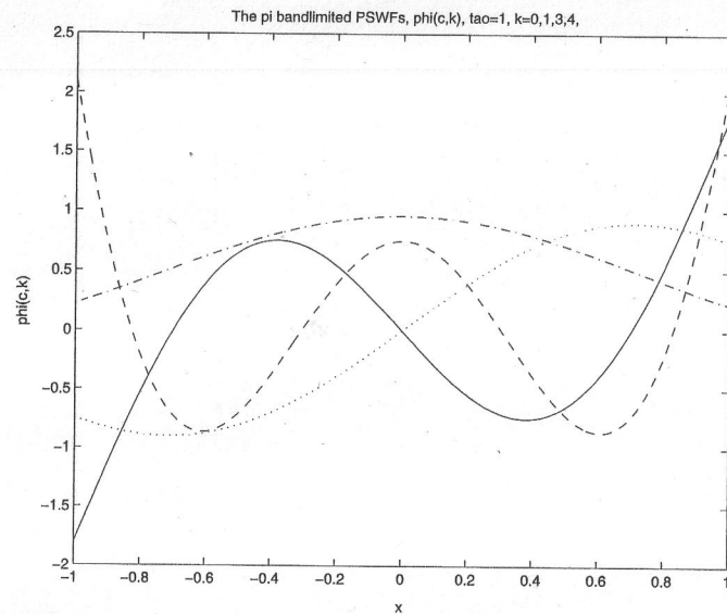
FIGURE 1. The PSWFs \varphi_0, \varphi_1, \varphi_3, \varphi_4 , with parameter values \sigma = \pi and \tau = 1 on the concentration interval [-1, 1] .
