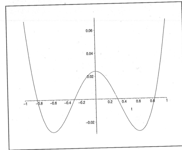
FIGURE 6. The polynomial approximation P_4 to \varphi_4 on the interval [-1, 1] .
