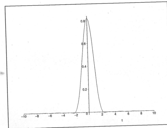
FIGURE 3. The PSWFs \varphi_0 with parameter values \sigma = \pi and \tau = 2 on a larger interval.
