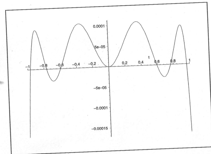
FIGURE 5. The error in the polynomial approximation to \varphi_0 on the interval [-1, 1] .
