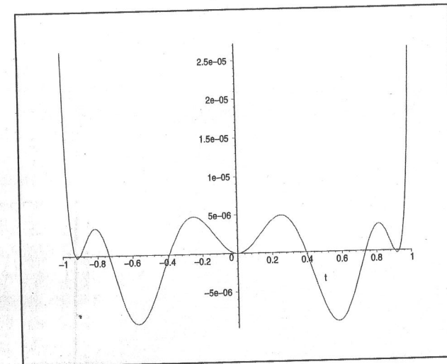
FIGURE 7. The error in the polynomial approximation to \varphi_4 on the interval [-1, 1] .
