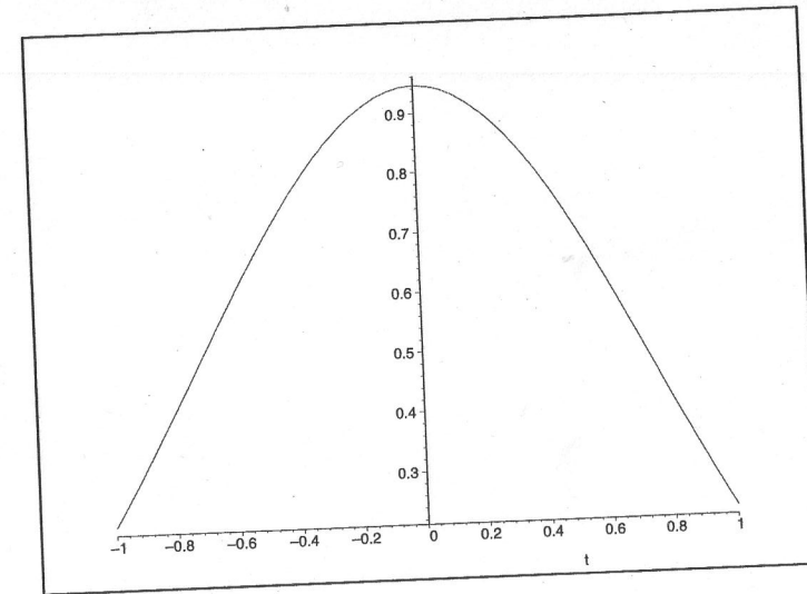
FIGURE 4. The Legendre polynomial P_0 approximation of degree 6 to \varphi_0 , \sigma = \pi , \tau = 1 on [-1, 1] .
