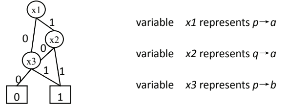
Figure 2. The BDD for \mathbb{C} = (p \rightarrow a \wedge q \rightarrow a) \vee p \rightarrow b .
