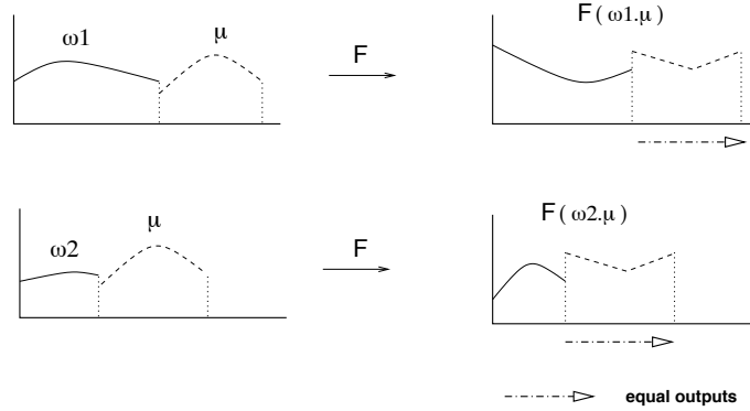
Fig. 2. Nerode Equivalence
