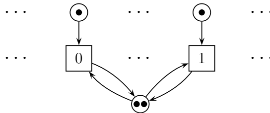
Fig. 2. A net without a \sqsubseteq_1^\infty -largest BD-process.
