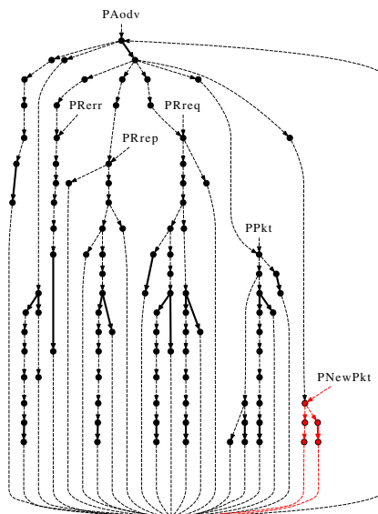
Fig. 3: Process term graph of \Gamma_{\text{aodv}}
