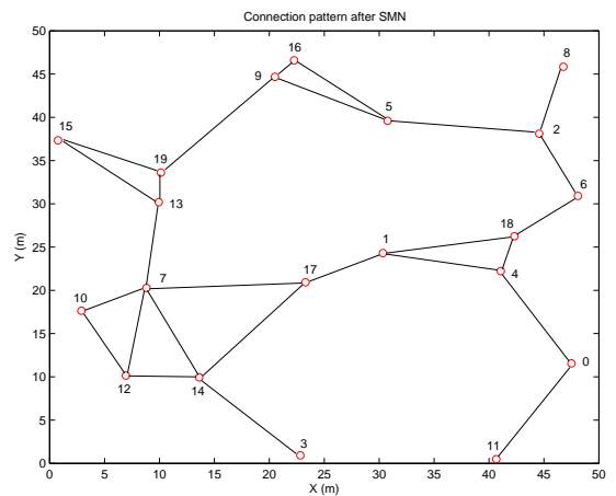
Fig. 21. Node connection pattern after using SMN
