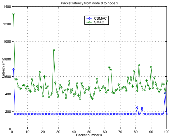
Fig. 12. Packet latency from node 0 to node 2
