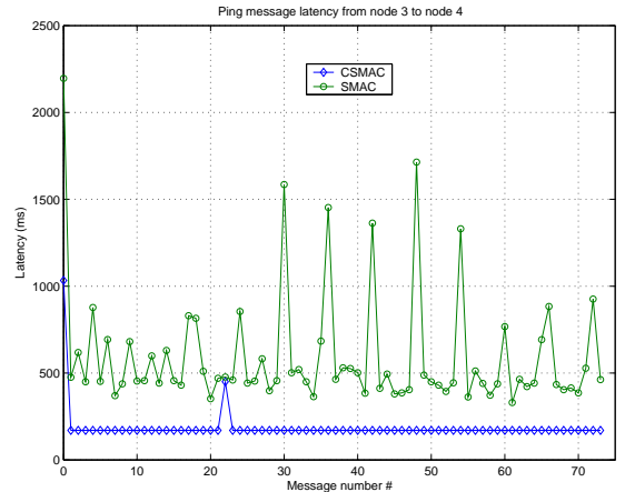
Fig. 16. Ping message latency from node 3 to node 4
