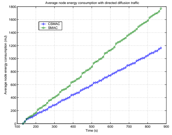
Fig. 14. Average node energy consumption with directed diffusion traffic
