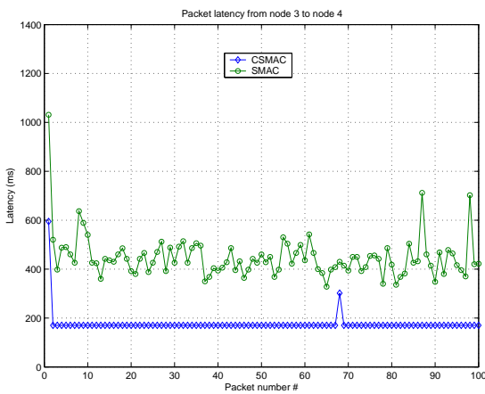
Fig. 13. Packet latency from node 3 to node 4
