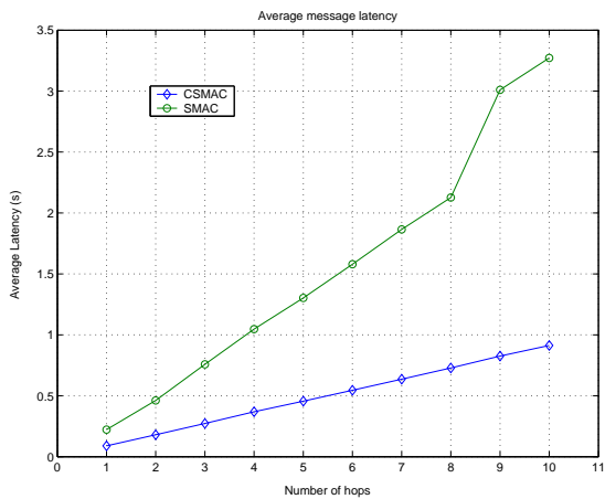
Fig. 19. Average message latency for 10 hops
