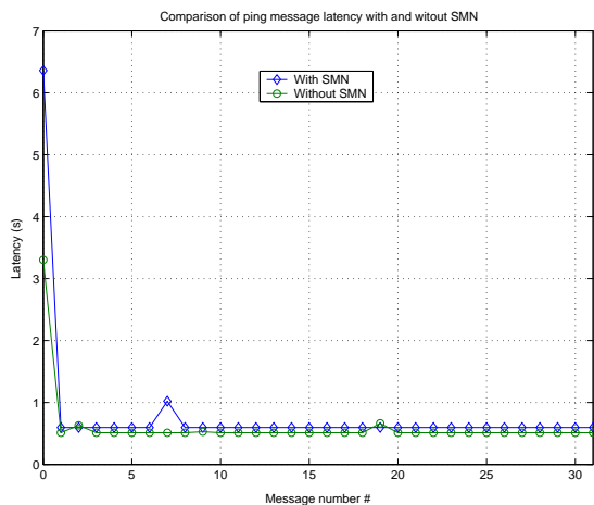
Fig. 24. Comparison of message latency with and without SMN from node 8 to node 10
