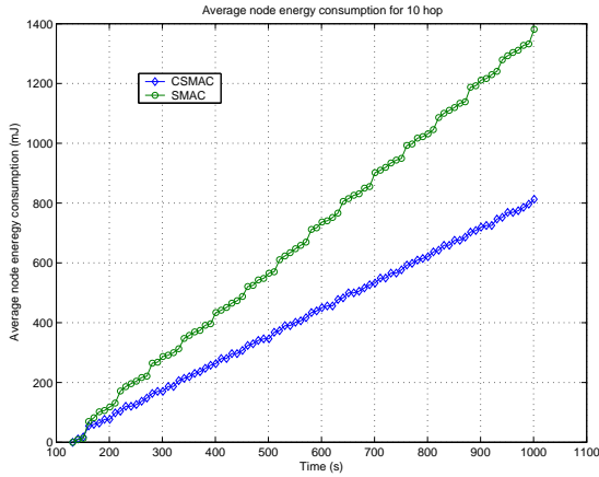
Fig. 18. Average node energy consumption for 10 hops
