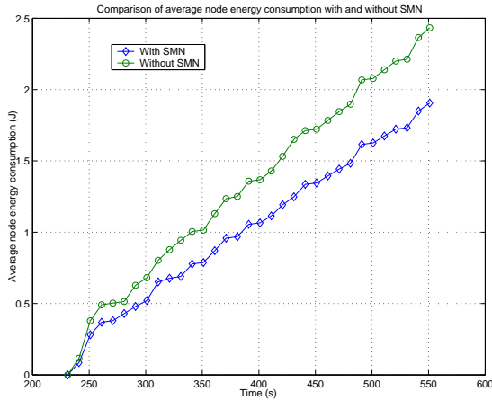
Fig. 22. Comparison of average energy consumption with and without SMN
