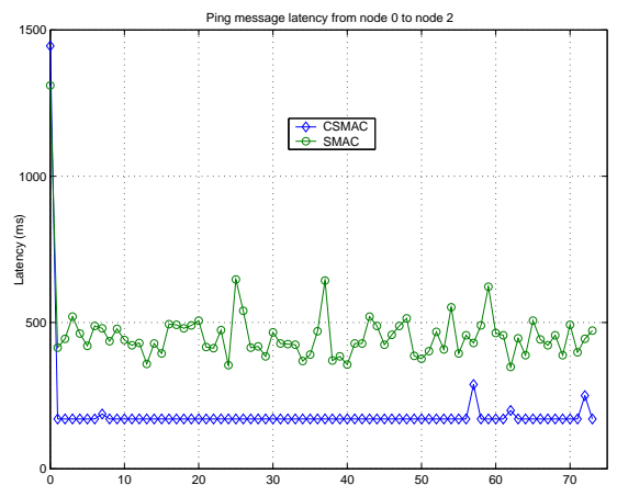
Fig. 15. Ping message latency from node 0 to node 2
