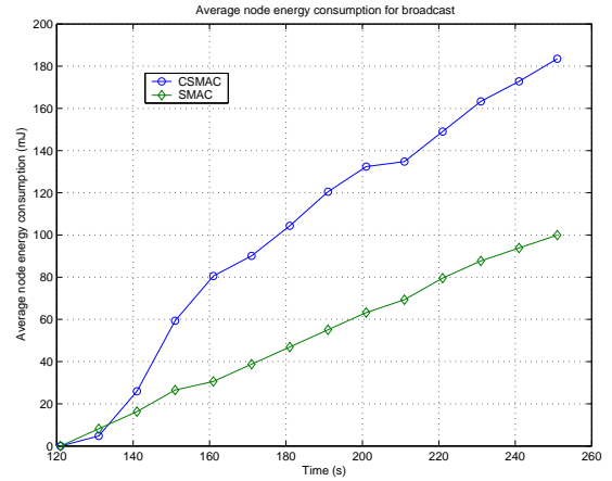
Fig. 10. Average per node energy consumption for broadcast traffic
