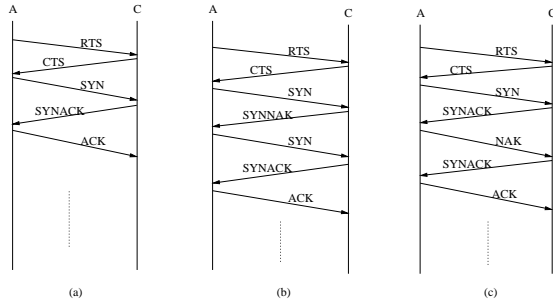
Fig. 7. (a) Normal Operation. (b) C disagrees with the PN code or Receiving Frequency of A. (c) A disagrees with the PN code or Receiving Frequency of C.
