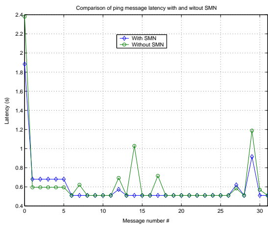
Fig. 23. Comparison of message latency with and without SMN from node 15 to node 0
