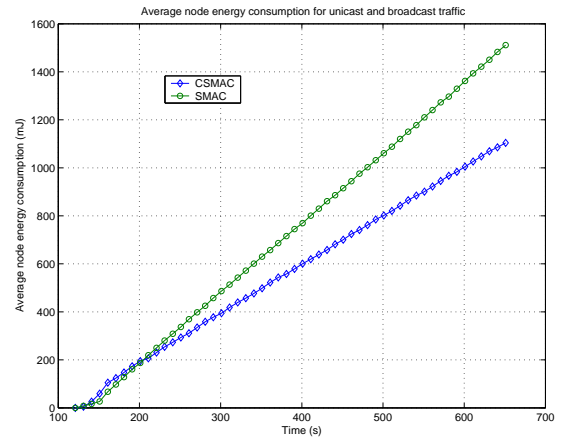
Fig. 11. Average per node energy consumption for both unicast and broadcast traffic
