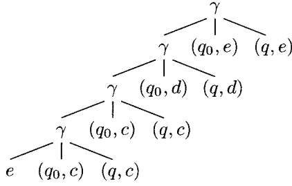
FIG. 4. The tree t = \tau_N(\#(d(c(c(e)))) .
