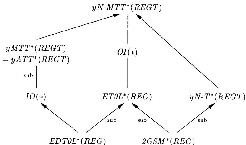
FIG. 6. Inclusions of hierarchies of string languages.
