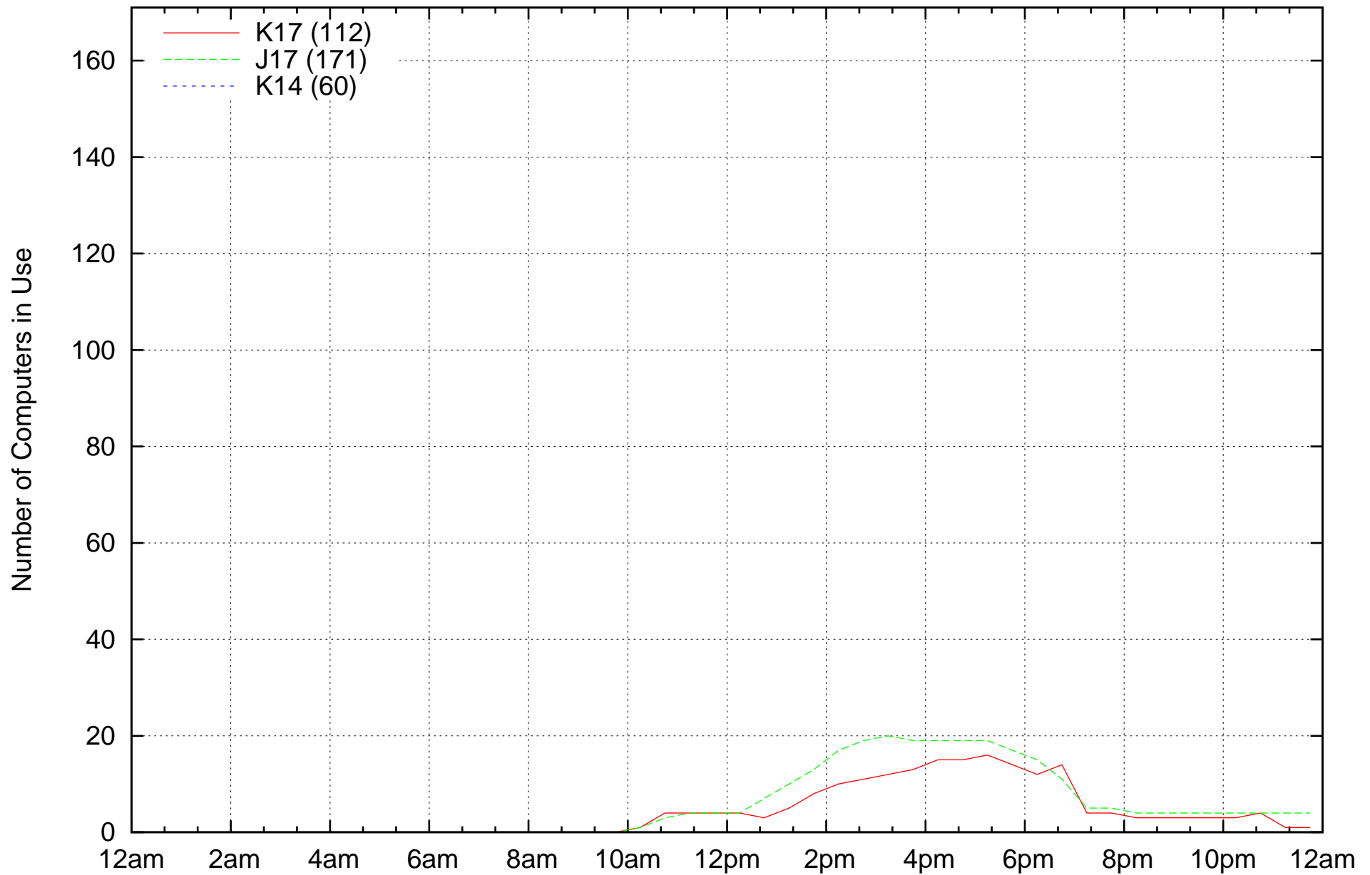
Total computer usage: 2019 Session 2, Week 11, Sunday 25 August 2019
