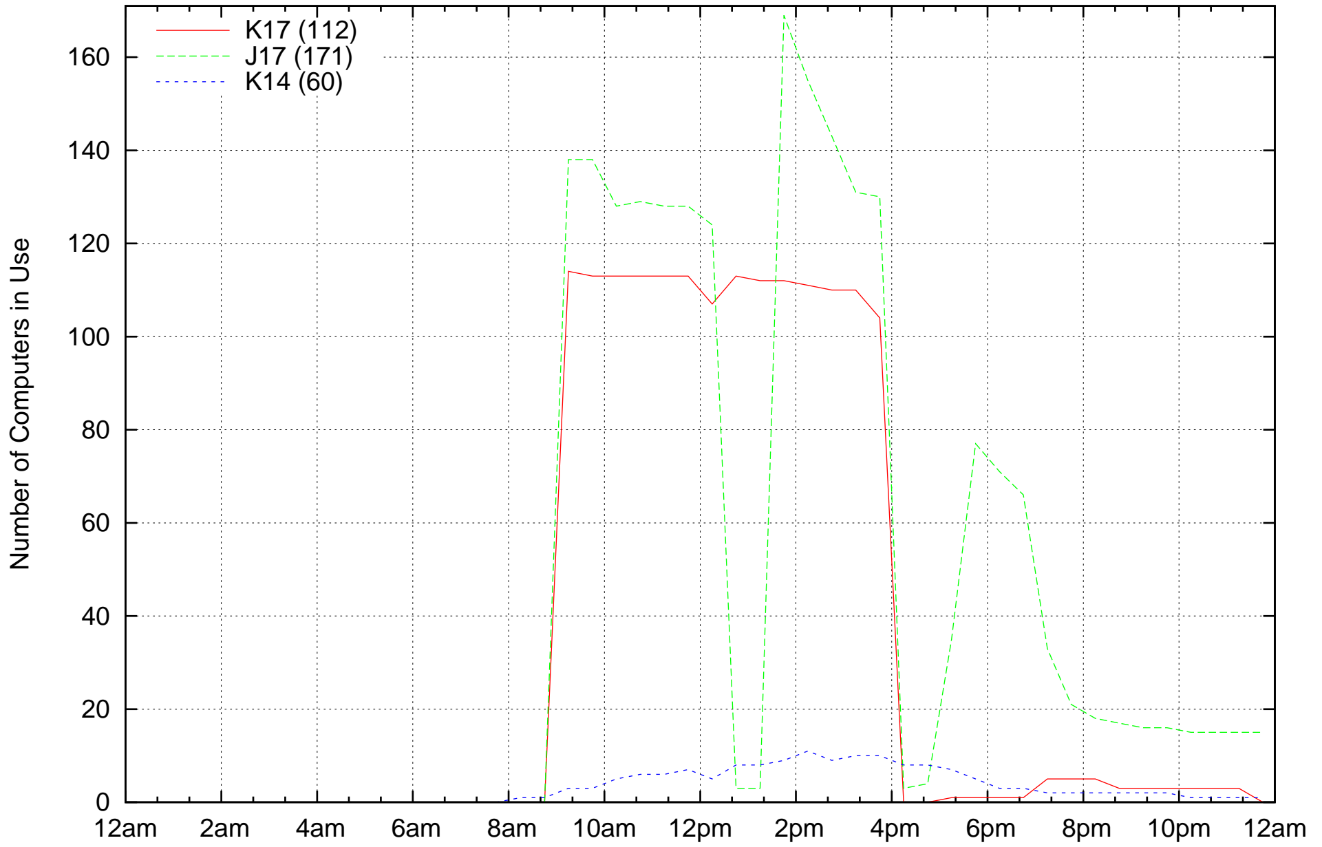
Total computer usage: 2019 Session 2, Week 12, Wednesday 28 August 2019
