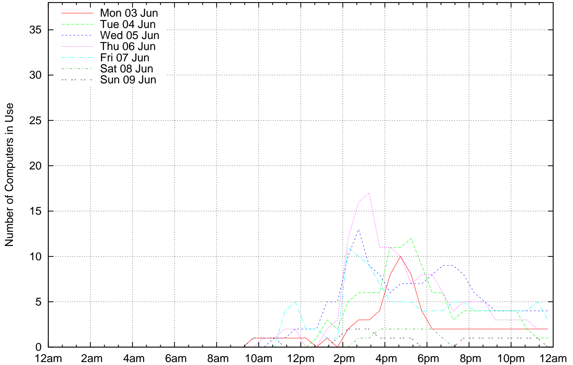
Lab usage: 2019 Session 2, Week 1, Special Labs (38 computers)
