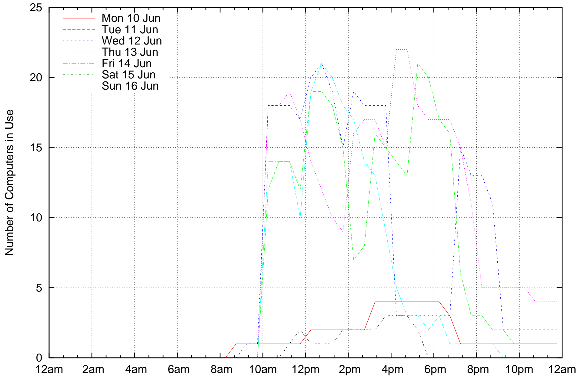
Lab usage: 2019 Session 2, Week 2, flute lab (25 computers)
