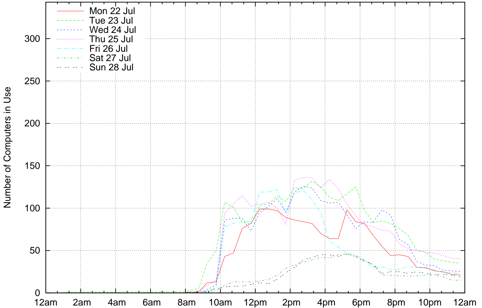
Lab usage: 2019 Session 2, Week 7, Combined Labs (343 computers)
