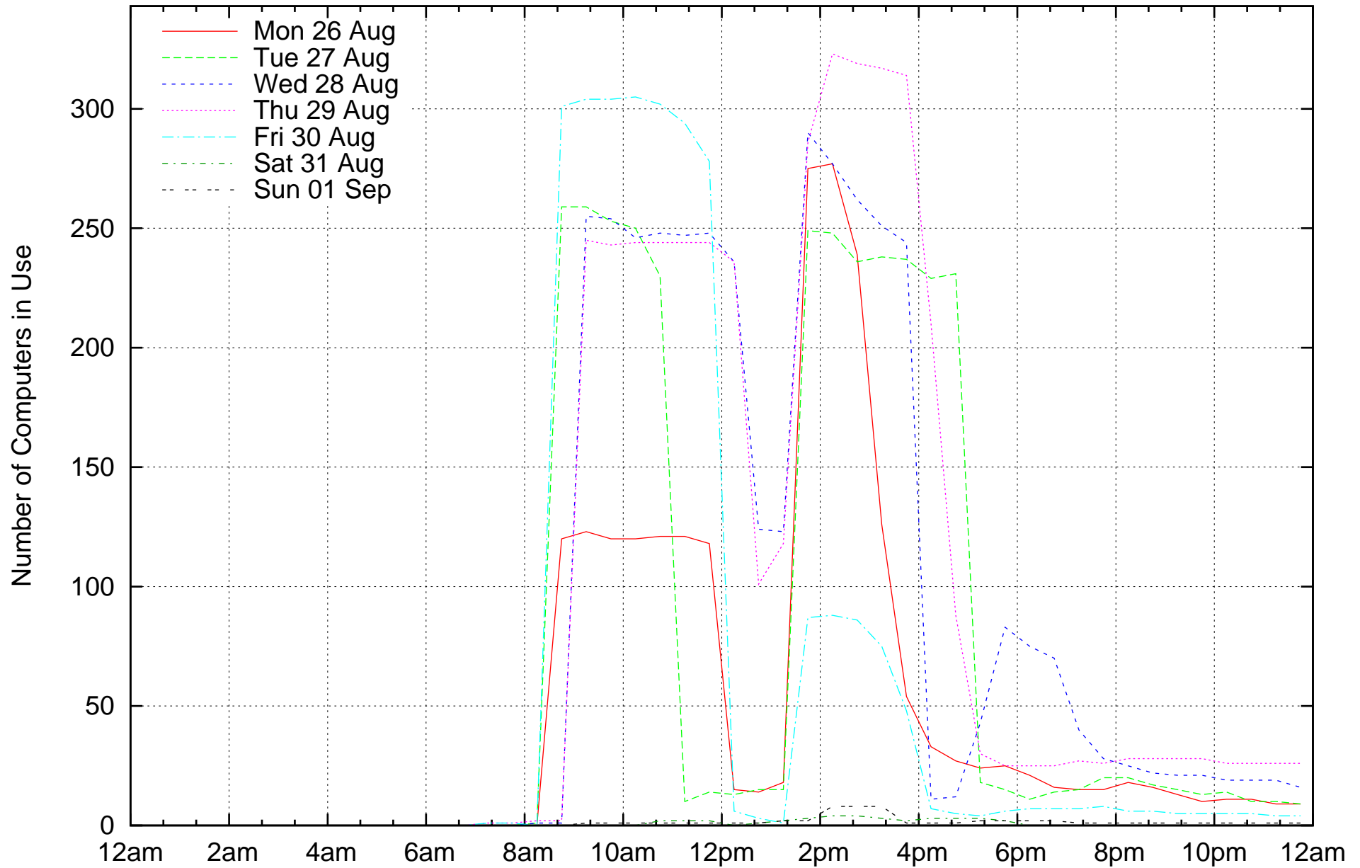
Lab usage: 2019 Session 2, Week 12, Combined Labs (343 computers)
