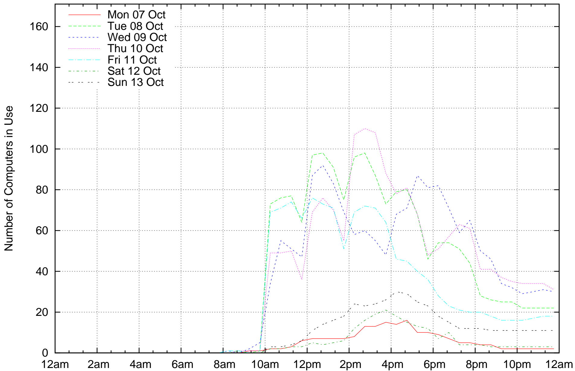
Lab usage: 2019 Session 3, Week 4, J17 (171 computers)
