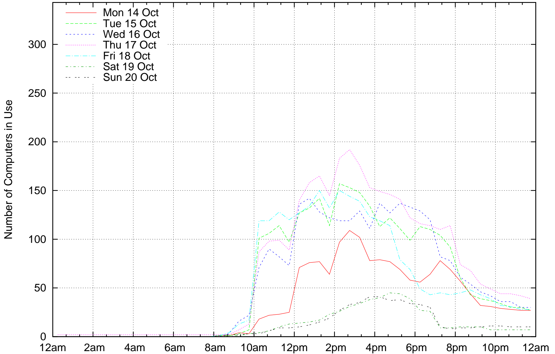
Lab usage: 2019 Session 3, Week 5, Combined Labs (343 computers)
