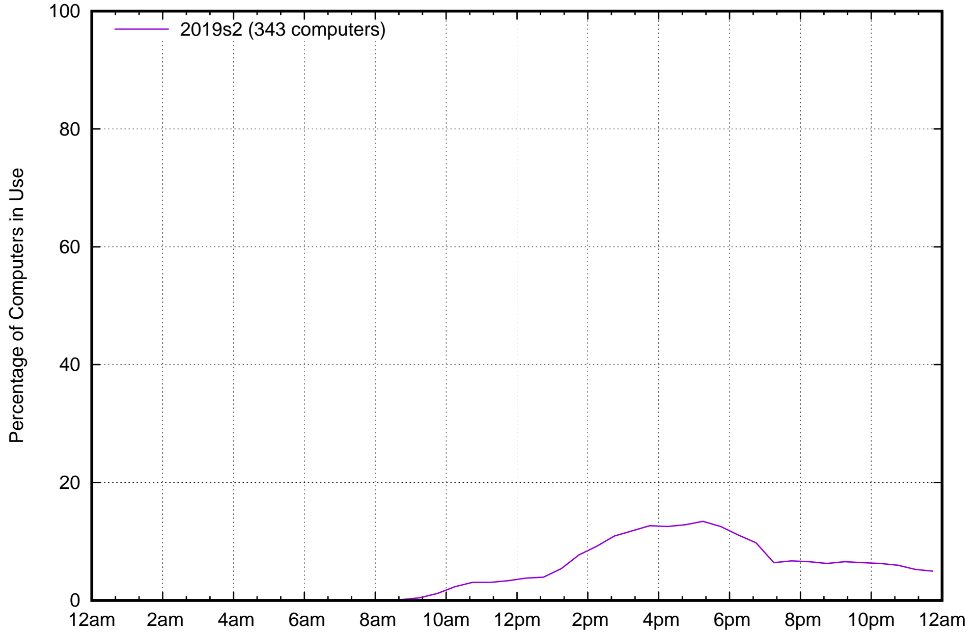
Percentage total use per day -- all labs, Session 2, Week 7, Week Ends
