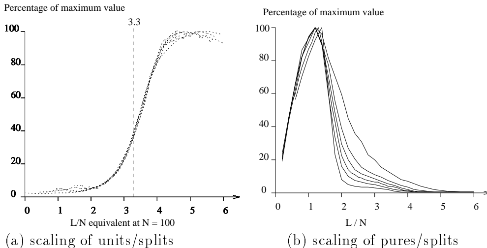
Figure 5: CP problems tested using DP, N = 25 to 300
