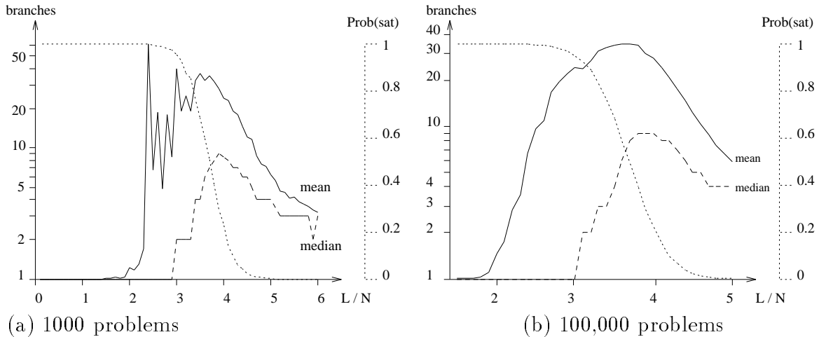
Figure 2: CP problems tested using DP, N = 100 . Mean and median branches
