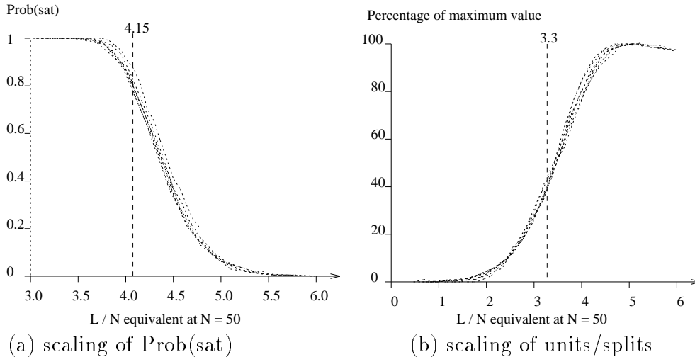
Figure 6: Random 3-SAT problems tested using DP, N = 10 to 70
