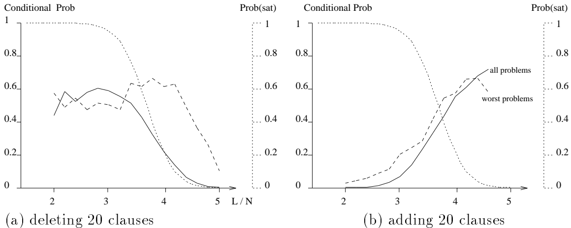
Figure 9: CP, 100 hardest sat/unsat problems for DP from 100,000, N=100
