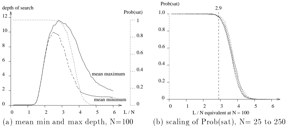
Figure 4: CP problems tested using DP.
