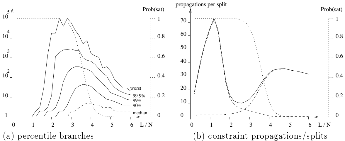
Figure 7: Random 2,4,4-SAT problems tested using DP, N=100 .
