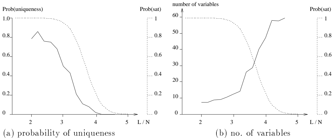
Figure 10: Minimal unsatisfiable subsets for 100 hardest unsat CP problems. N = 100
