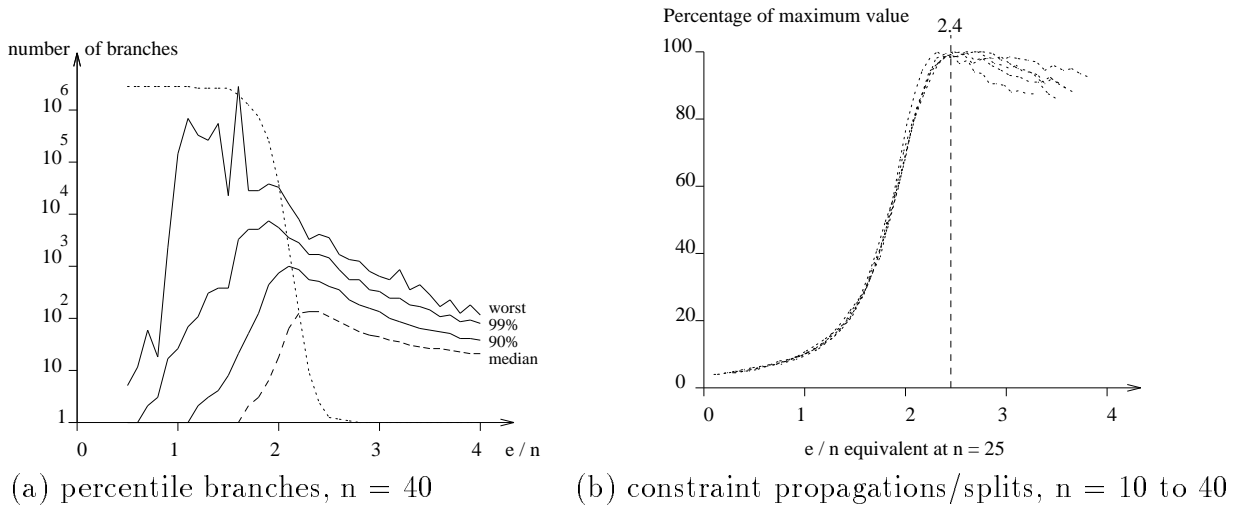
Figure 8: 3COL problems from \chi(n, e) tested with DP
