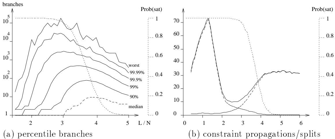
Figure 3: CP problems tested using DP, N= 100 .
