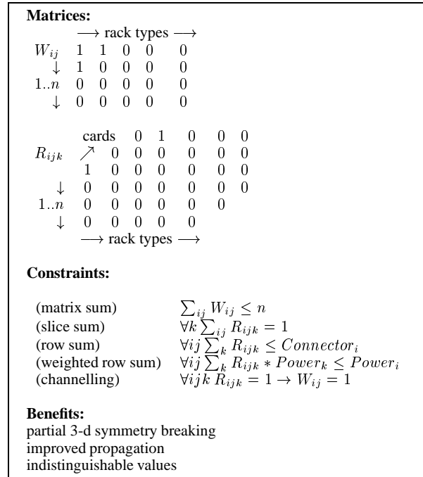
Figure 2: Matrix model for the rack configuration problem
