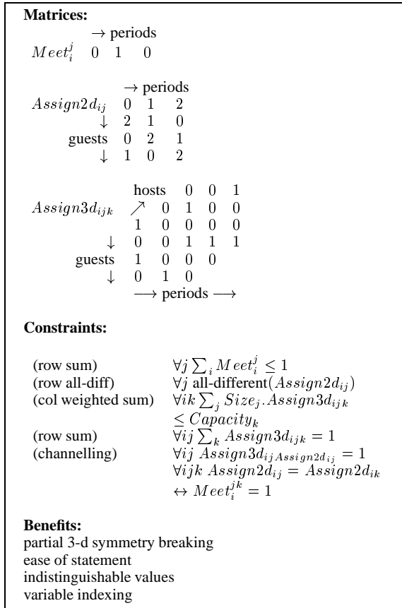
Figure 7: Matrix model for the progressive party problem
