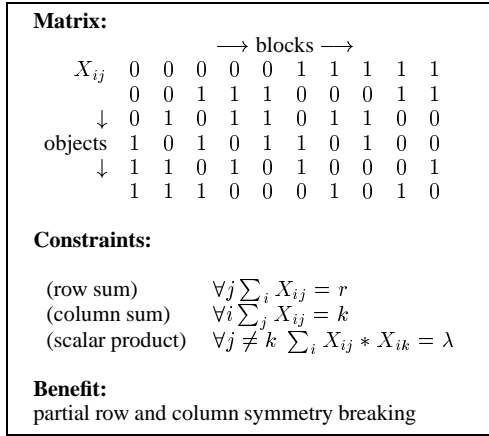
Figure 1: Matrix model for the BIBD generation problem
