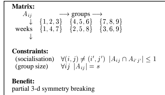
Figure 3: Matrix model for the social golfers problem
