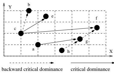
Figure 10. A CBC Dominance Graph
