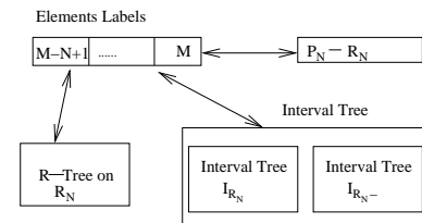
Figure 11. Data Structure Maintained
