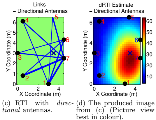
Figure 2: Omni-directional RTI vs dRTI. The thicknesses of lines in (a) and (c) are proportional to the vRTI link quality statistics. The crosses (×) show the true location of the obstruction. Fig. (b) shows that the RTI image with a large localisation error because of a deep fade between Nodes 2 and 5 in (a). However, this fade has little impact on dRTI estimation shown in (d).
