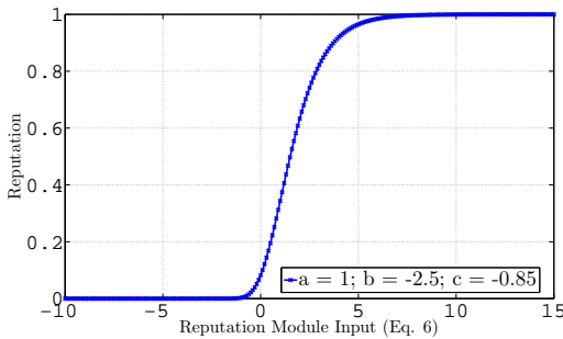
Figure 4: Gompertz function
