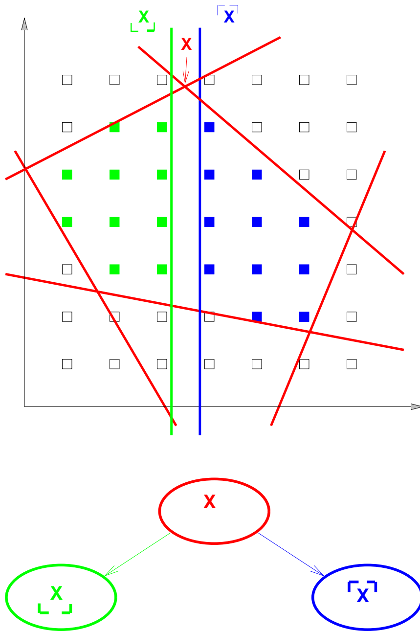
Figure 11 Branch-and-bound solution to the MIP problem
