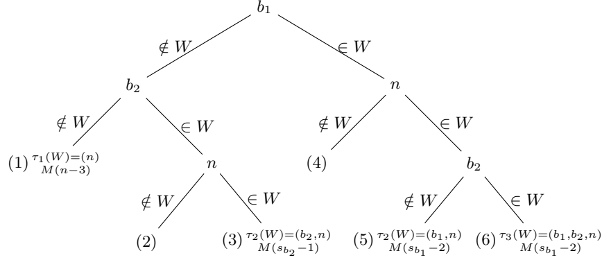
Fig. 2. Different possibilities for a maximal transitive vertex set W .
