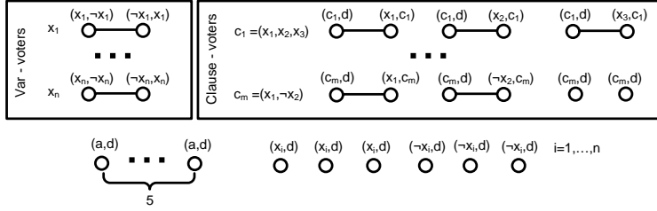
Figure 3: The construction from Theorem 7
