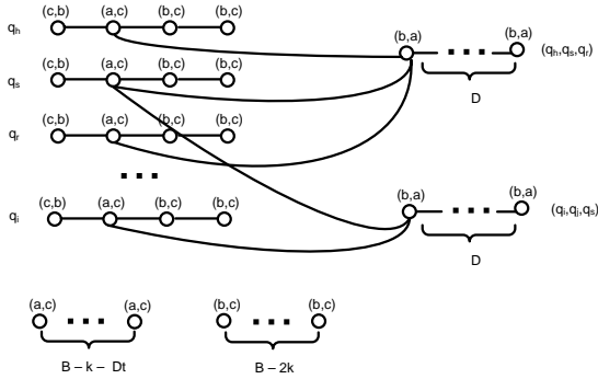
Figure 2: The construction from Theorem 5
