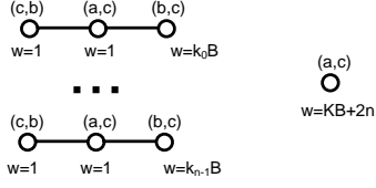
Figure 1: The construction from Theorem 4
